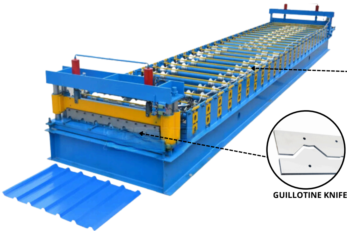
FORMING ROLLS
